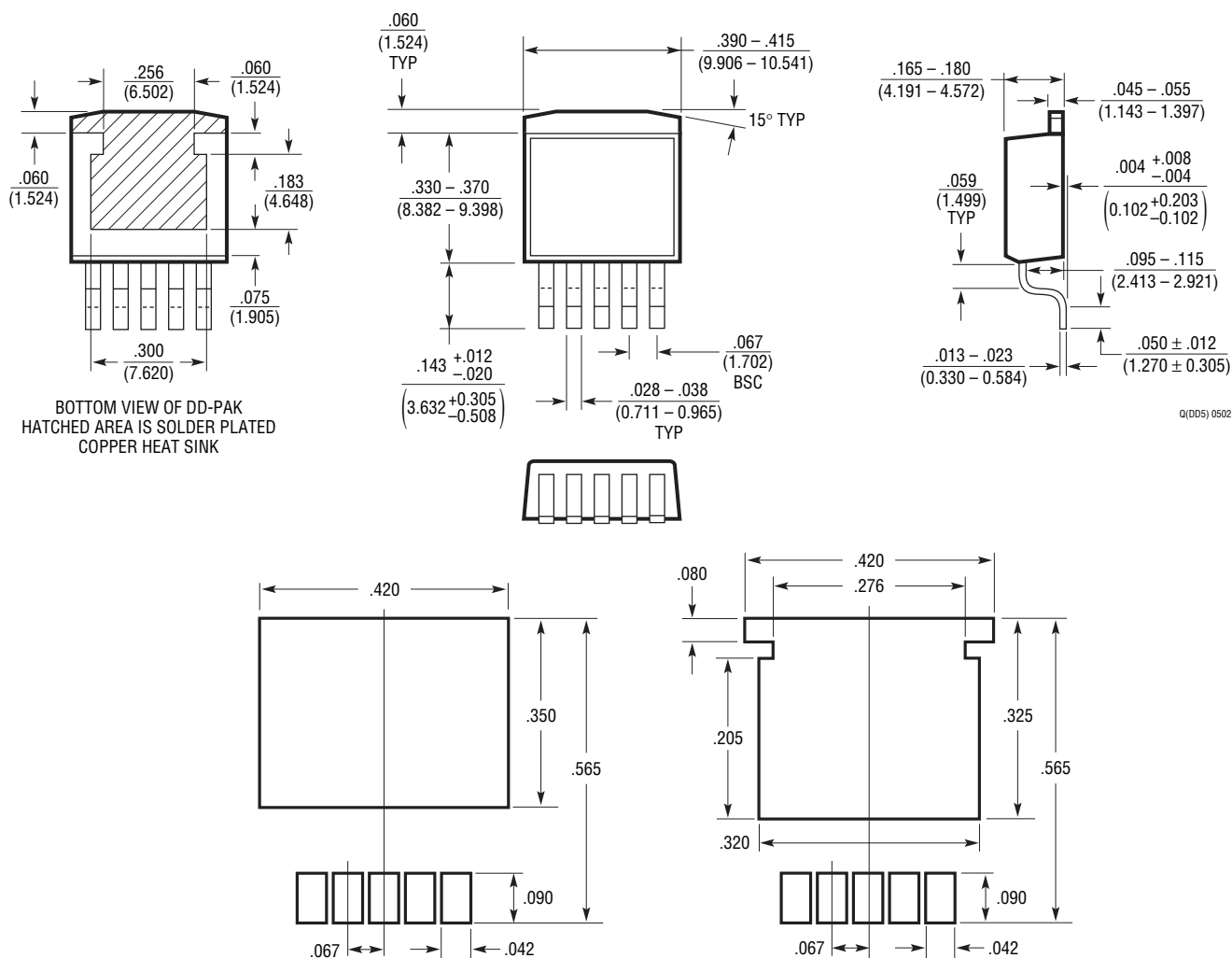
Q Package 5-Lead Plastic DD-Pak (Reference LTC DWG # 05-08-1461)
